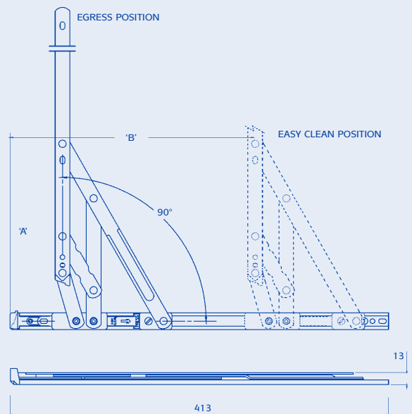
Defender 16” Easy Clean Egress Hinge
